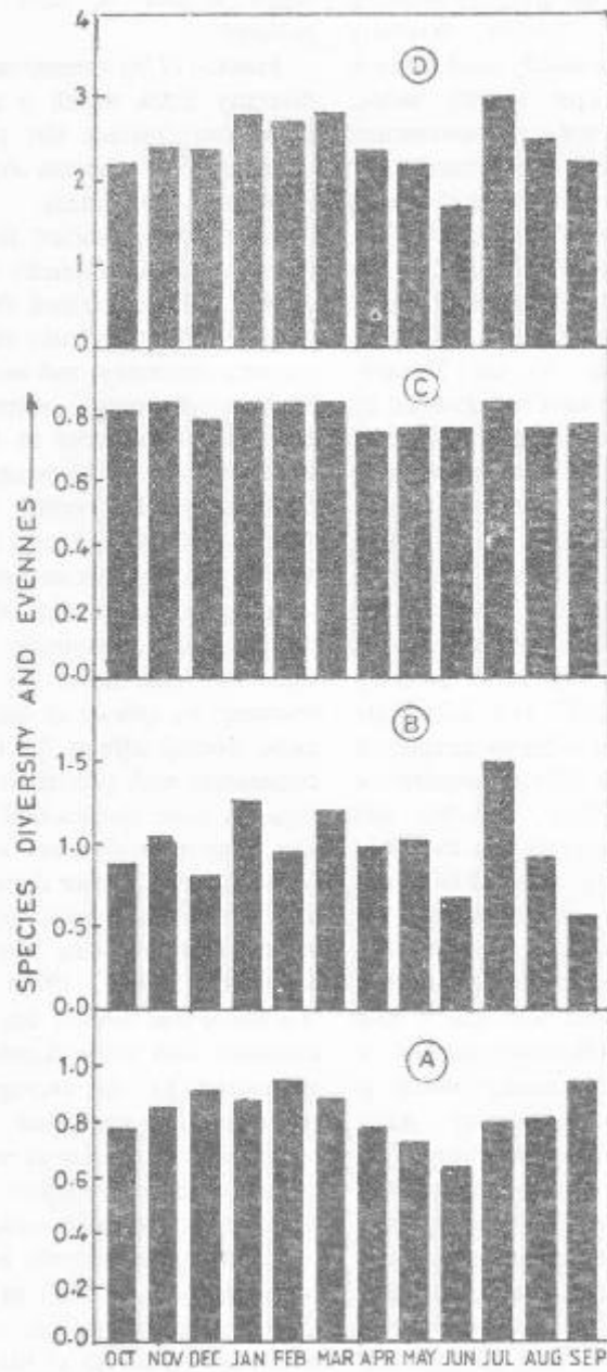
Fig. 1. Seasonal variation in evenness A, and species diversity indices by margalef B, by Simpson C, & by Shanon-Weaver D, formulae.
